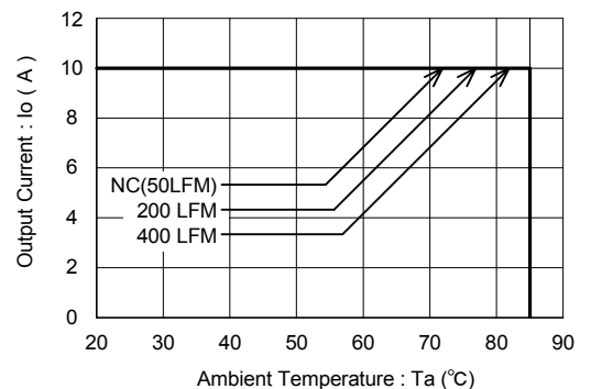
Figure15 BST12L-0.7S10PDM ( V_{in}=12.0V , V_o=1.0V )
