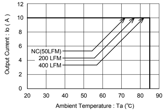
Figure14 BST12L-0.7S10PDM( V_{in}=12.0V , V_o=3.3V )
