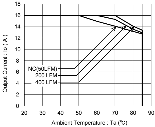
Figure16 BST12L-0.7S16PDM( Vin=12.0V, Vo=5.0V )
