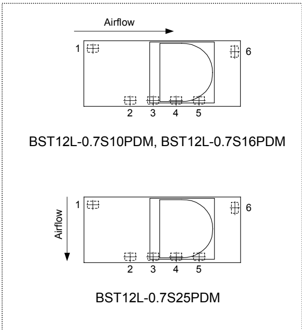
Figure 12. Temp derating air-cooling direction
