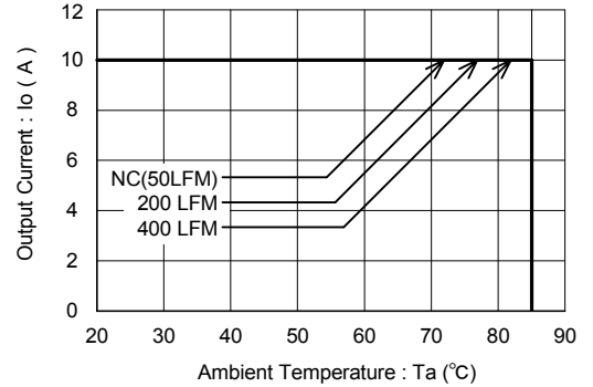
Figure13 BST12L-0.7S10PDM( V_{in}=12.0V , V_o=5.0V )
