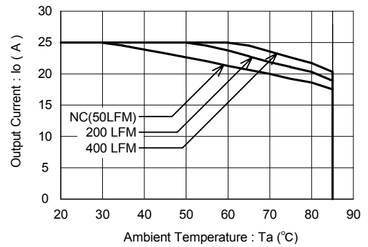
Figure20 BST12L-0.7S25PDM ( Vin=12.0V, Vo=3.3V )
