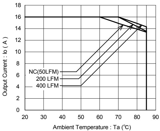
Figure17 BST12L-0.7S16PDM( Vin=12.0V, Vo=3.3V )
