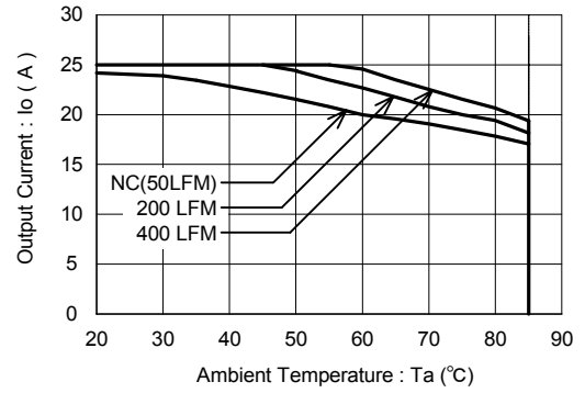
Figure19 BST12L-0.7S25PDM ( Vin=12.0V, Vo=5.0V )
