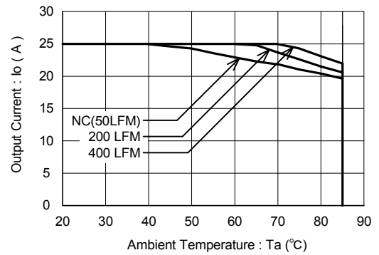
Figure21 BST12L-0.7S25PDM( Vin=12.0V, Vo=1.0V )
