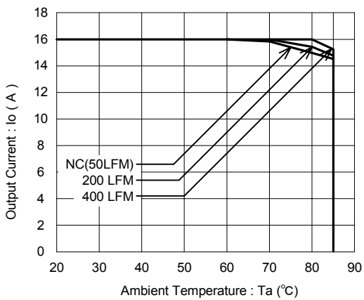
Figure18 BST12L-0.7S16PDM( Vin=12.0V, Vo=1.0V )
